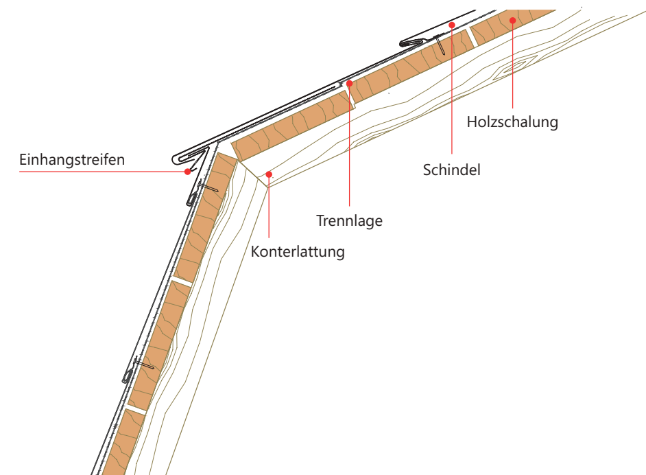
DETAIL MANSARDENKNICK
