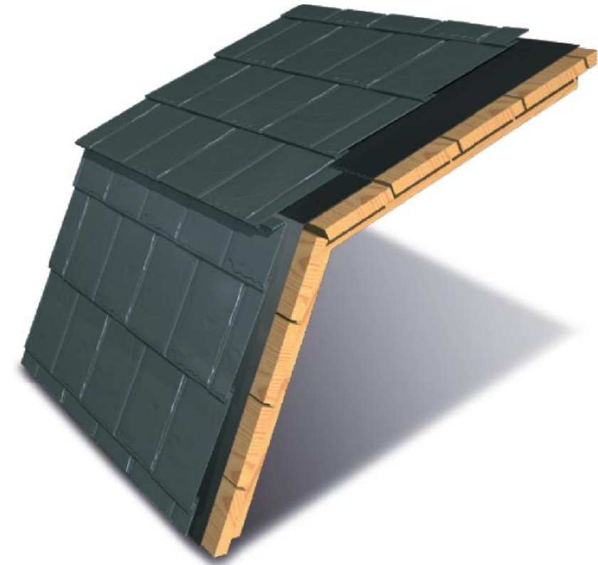
DETAIL MANSARDENKNICK
