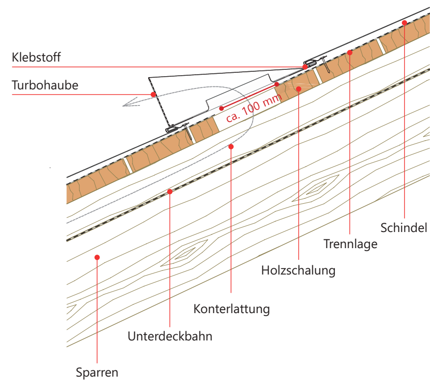
DETAIL TURBOHAUBE
