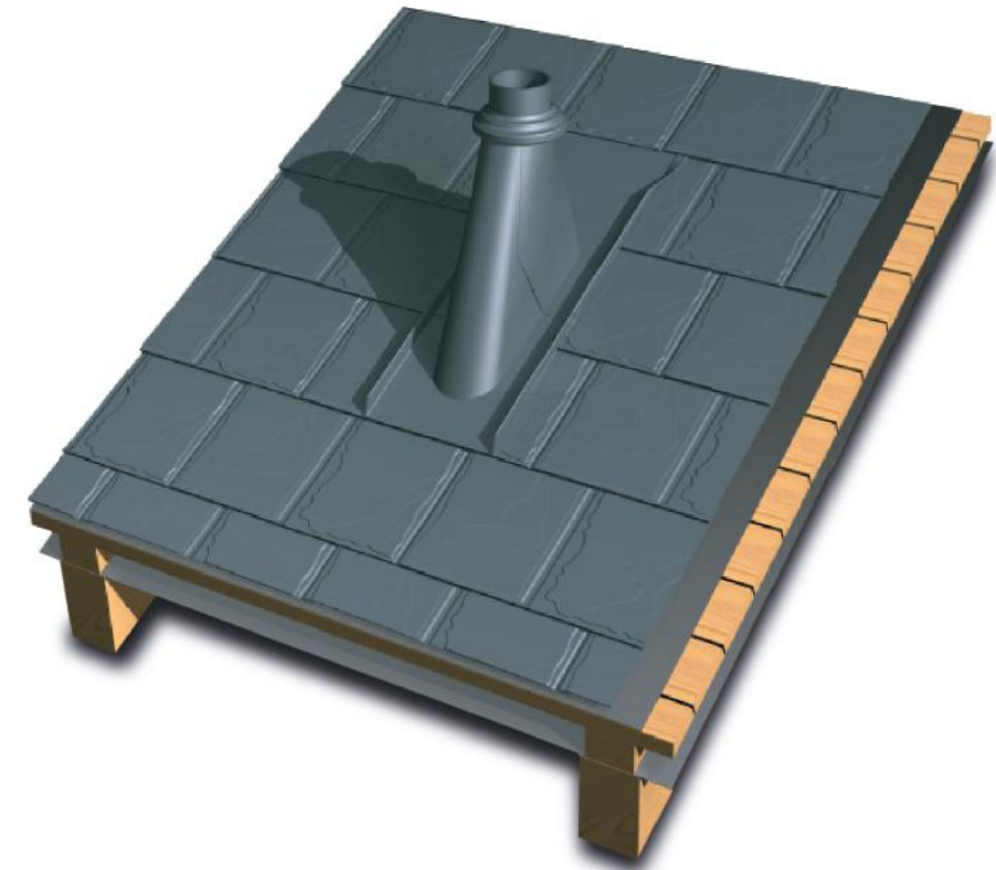
DETAIL DUNSTROHR
